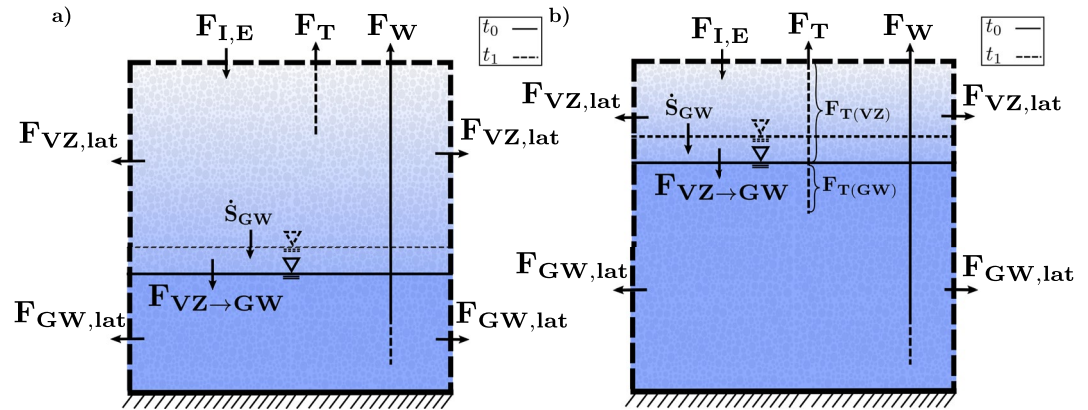
Figure 2. Fluxes in an integrated subsurface-flow model at two different times t_0 and t_1 . Illustrated are: The exchange flux at the land surface F_{I,E} , transpiration F_T , lateral in- and outflow from the vadose F_{VZ,lat} and phreatic F_{GW,lat} zones, the flux crossing the water table F_{VZ \rightarrow GW} , temporal groundwater-storage changes \dot{S}_{GW} , and the flux caused by an extraction well F_W . Arrows indicate the positive flow direction. Compressibility is not shown. (a) The water table lies below the root zone. Transpiration only drains the vadose zone. (b) The water table lies within the root zone. Transpiration is divided into transpiration of groundwater F_{T(GW)} and transpiration of soil water F_{T(S)} .
